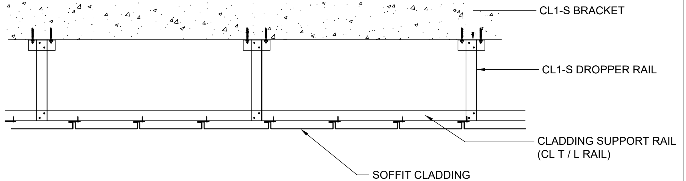
CL1-S TYPICAL ARRANGEMENT
