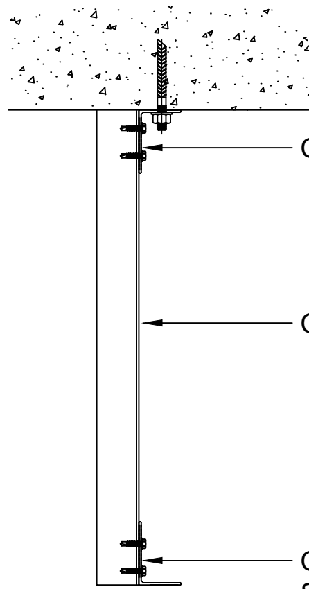
TYPICAL SECTION
