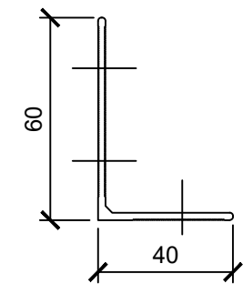
CL1-S BRACKET SECTION
