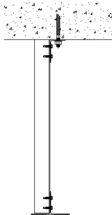
TYPICAL SECTION
